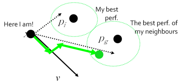
Figure 4.3: PSO position update.
