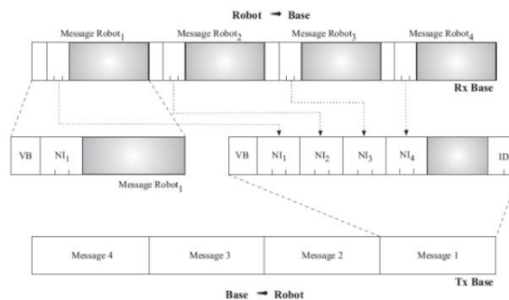
Figure 6.33: Packet format of the messages from and to the robots.
