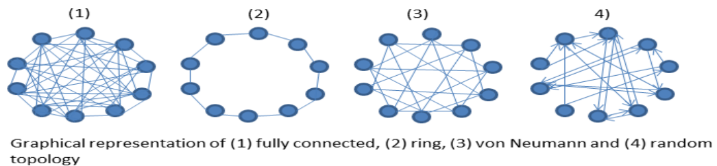
Figure 4.5: PSO topologies [57].
