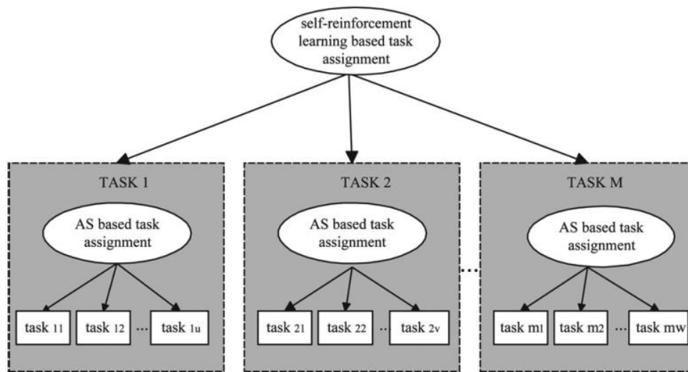
Figure 4.1: Architecture of the relationship among tasks
